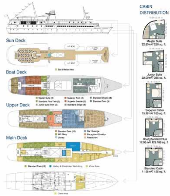
Main Deck
